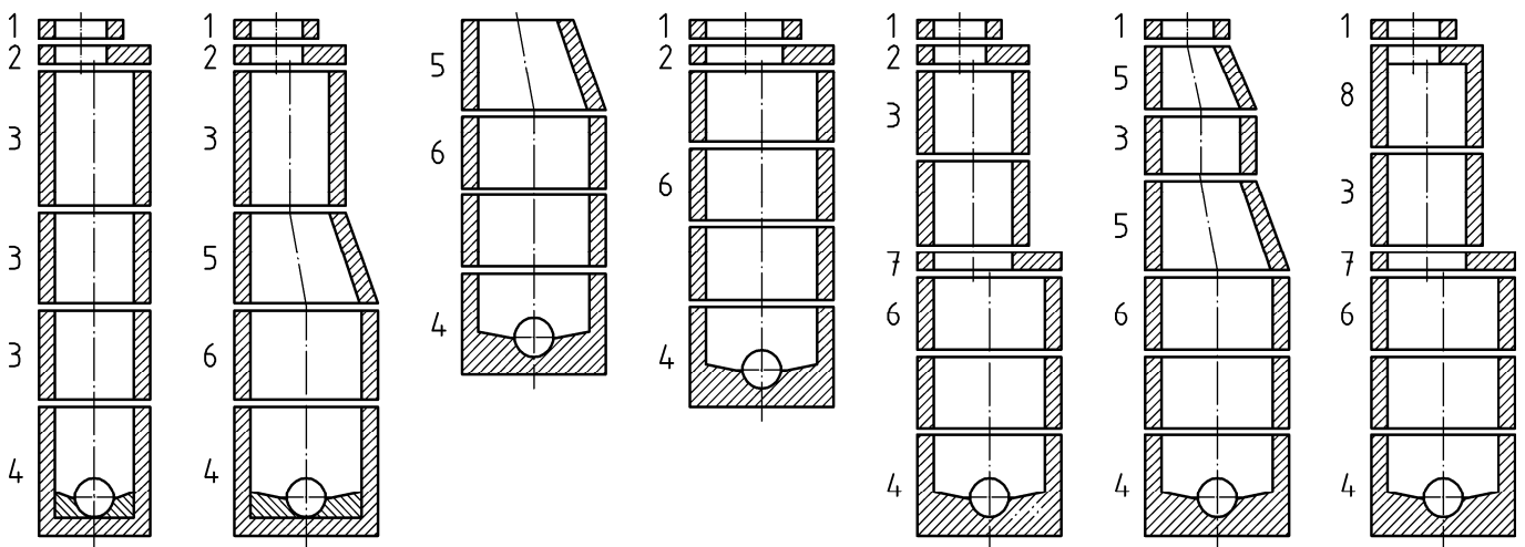
Figure 1 — Ouvrages types
